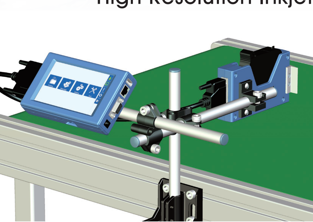
Elfin ID High Resolution Inkjet Printer
